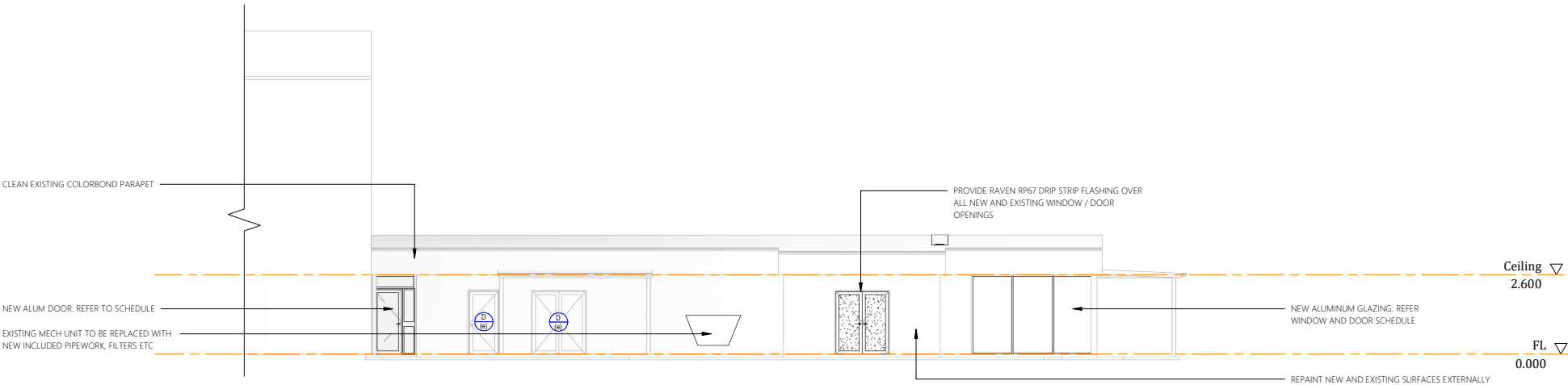
Proposed Elevation 1 1 : 100
