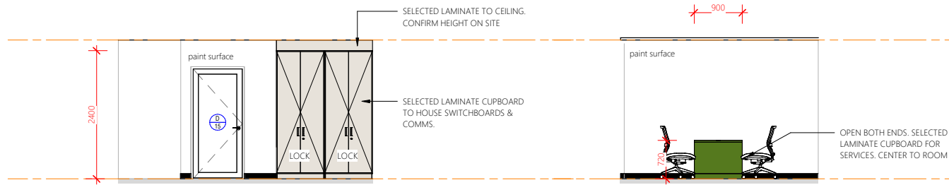
Elevation 2C 1:50
