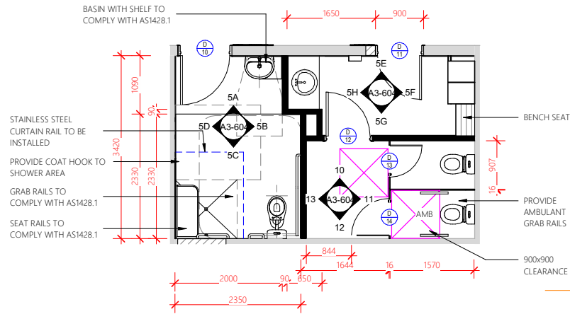
Internal Plan 5
