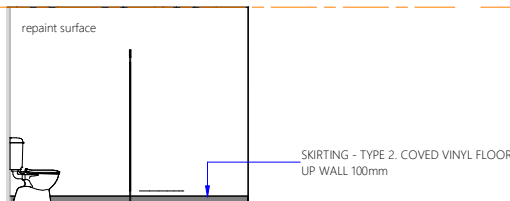
Elevation 5K
