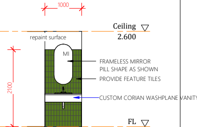
Elevation 5H
