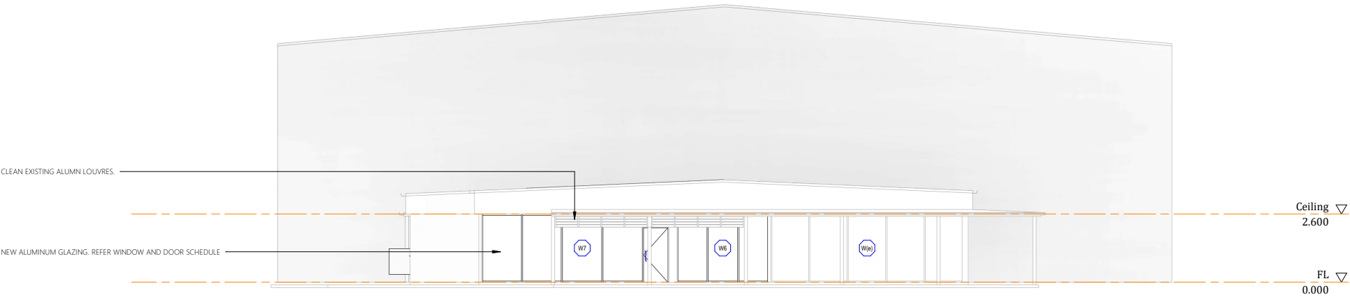
Proposed Elevation 2 1 : 100
