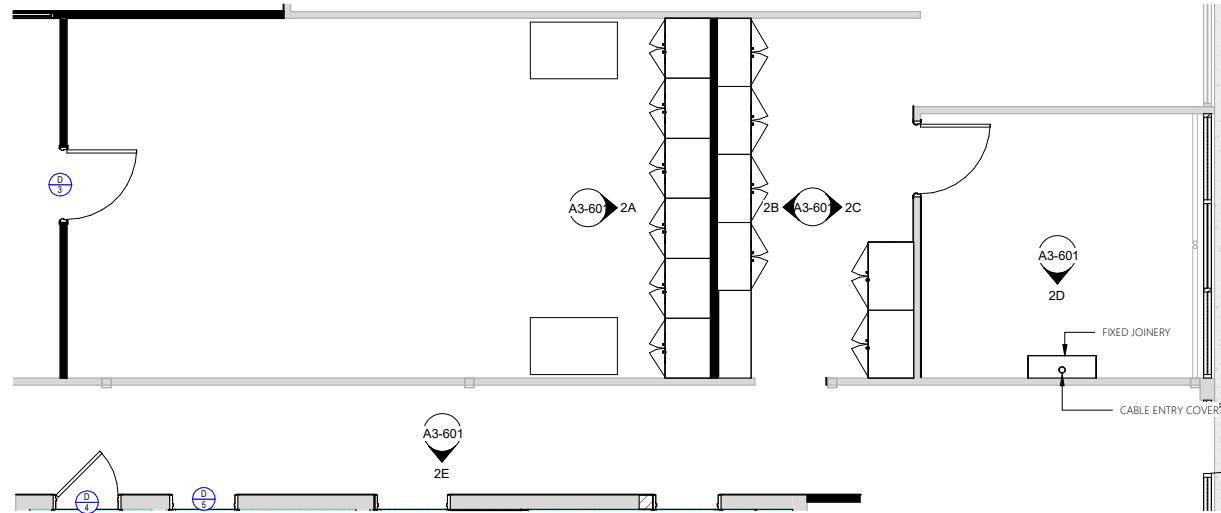
Internal Plan 2 1:50
